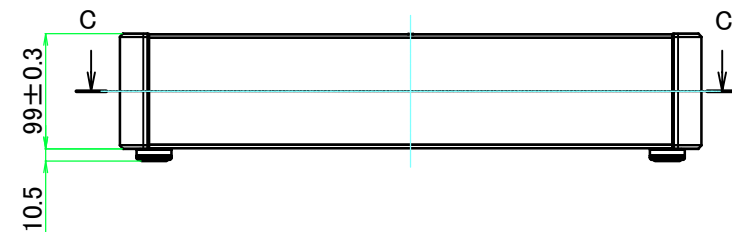
A view
